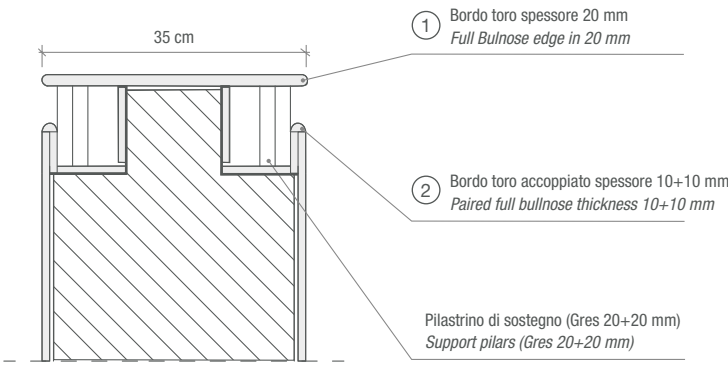
SWIMMING POOL-EDGE Carriere du Kronos Namur FLOOR Carriere du Kronos Namur 20,2x20,2 - 20,2x30,2
