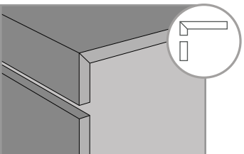
“ELLE SOSPESA” SUSPENDED L-SHAPE
